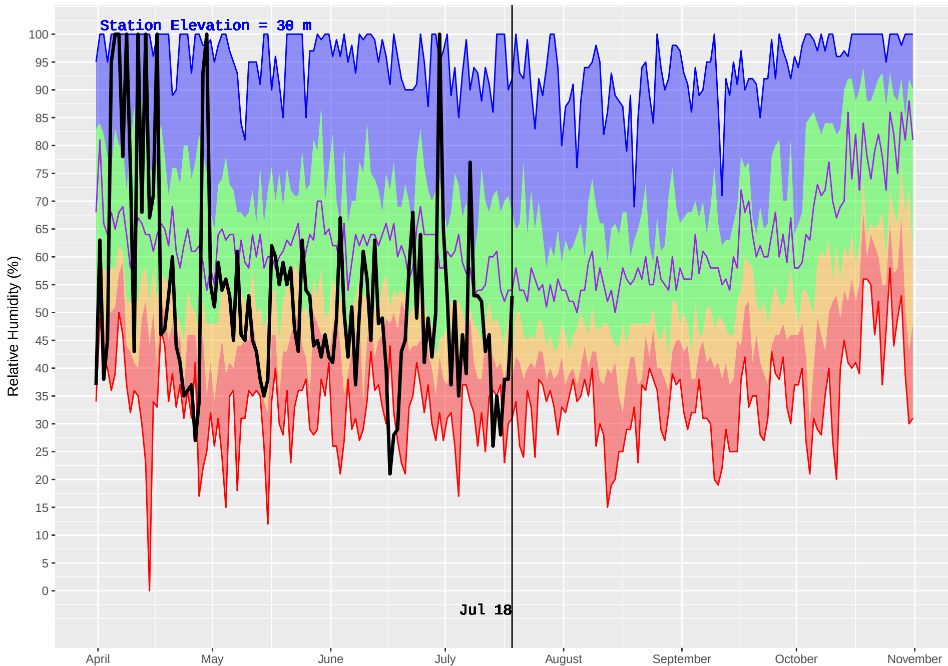
CEDAR (59) : Historical (1989–2016) and Current (2018) Daily Relative Humidity
