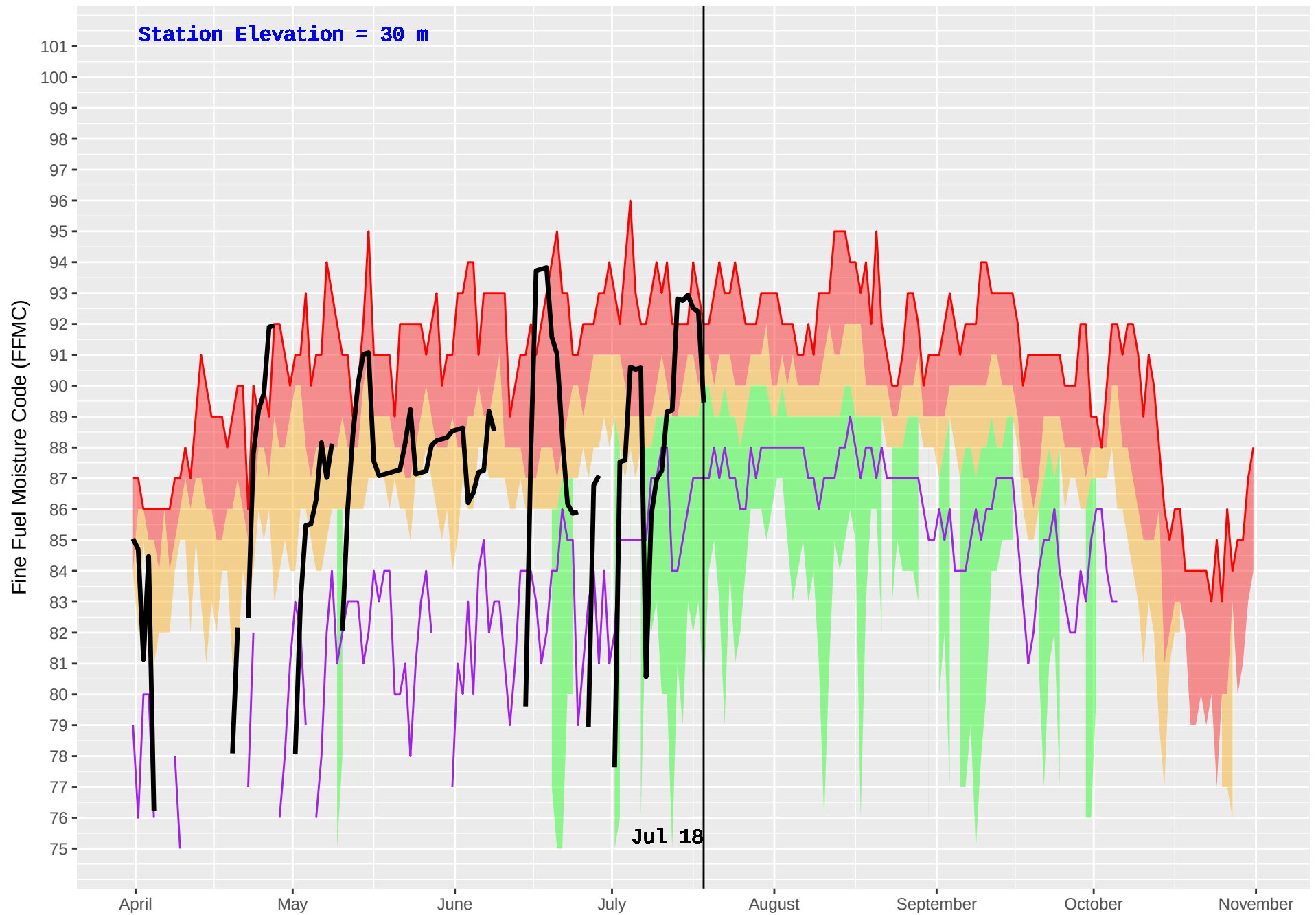
CEDAR (59) : Historical (1989–2016) and Current (2018) Daily Fine Fuel Moisture Code (FFMC)
