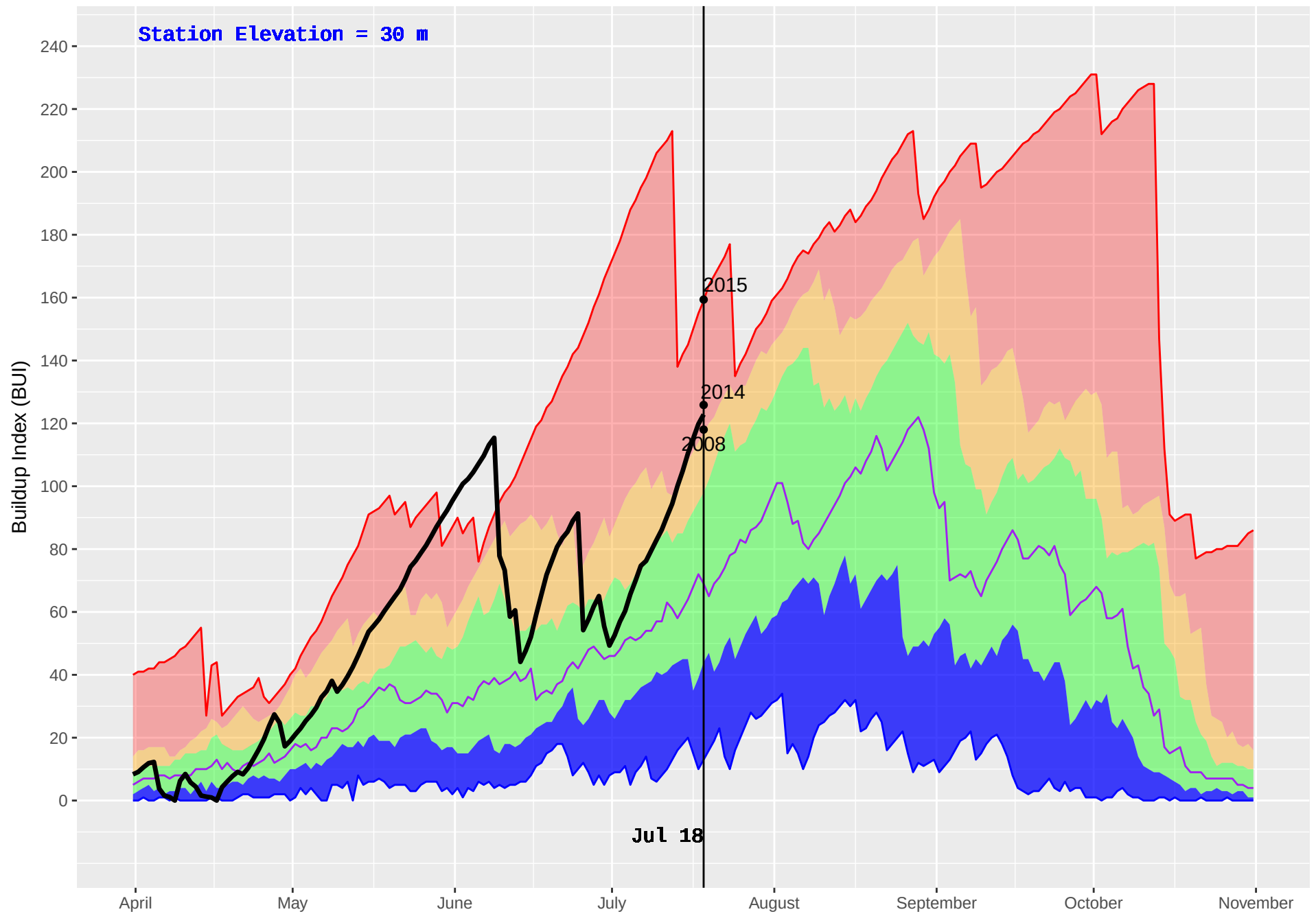
CEDAR (59) : Historical (1989–2016) and Current (2018) Daily Buildup Index (BUI)
